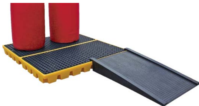
BFFE4 WITH BFFER RAMP
