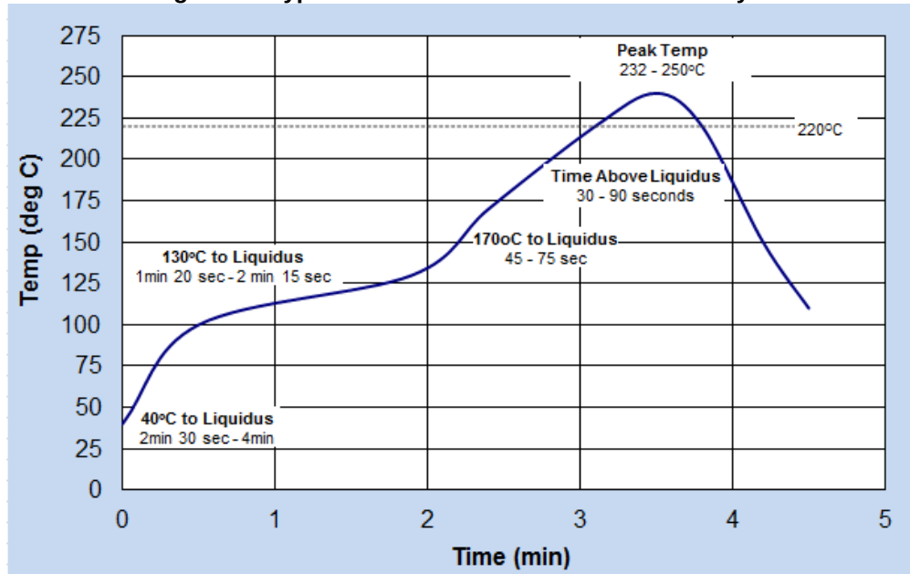
Figure 1: Typical Soak Reflow Profile for SAC Alloys
