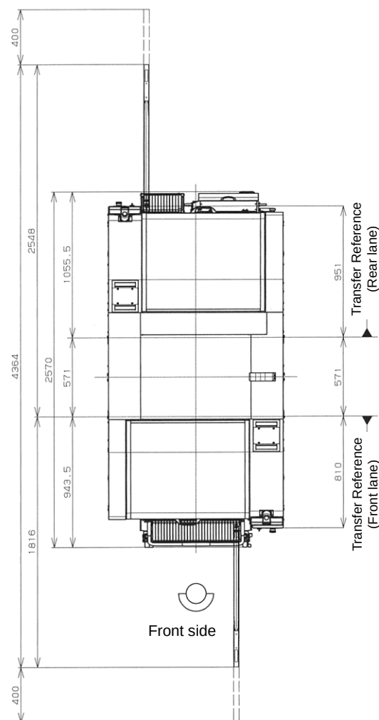
Dual conveyor specification
