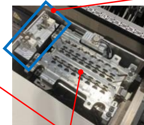
Nozzle holder pallet
